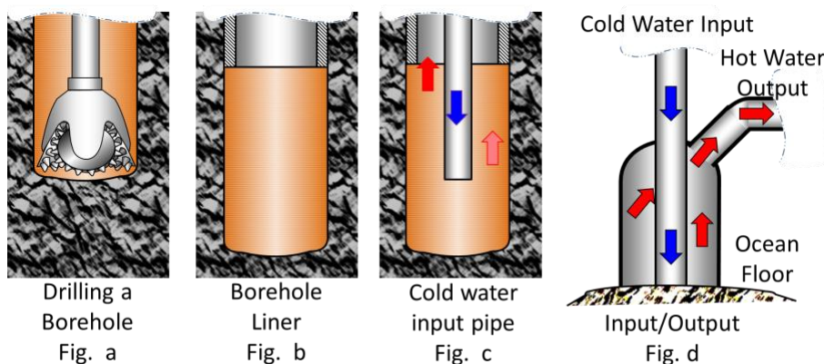
Figure 5 – Construction of a Hydrothermal Borehole Vent
