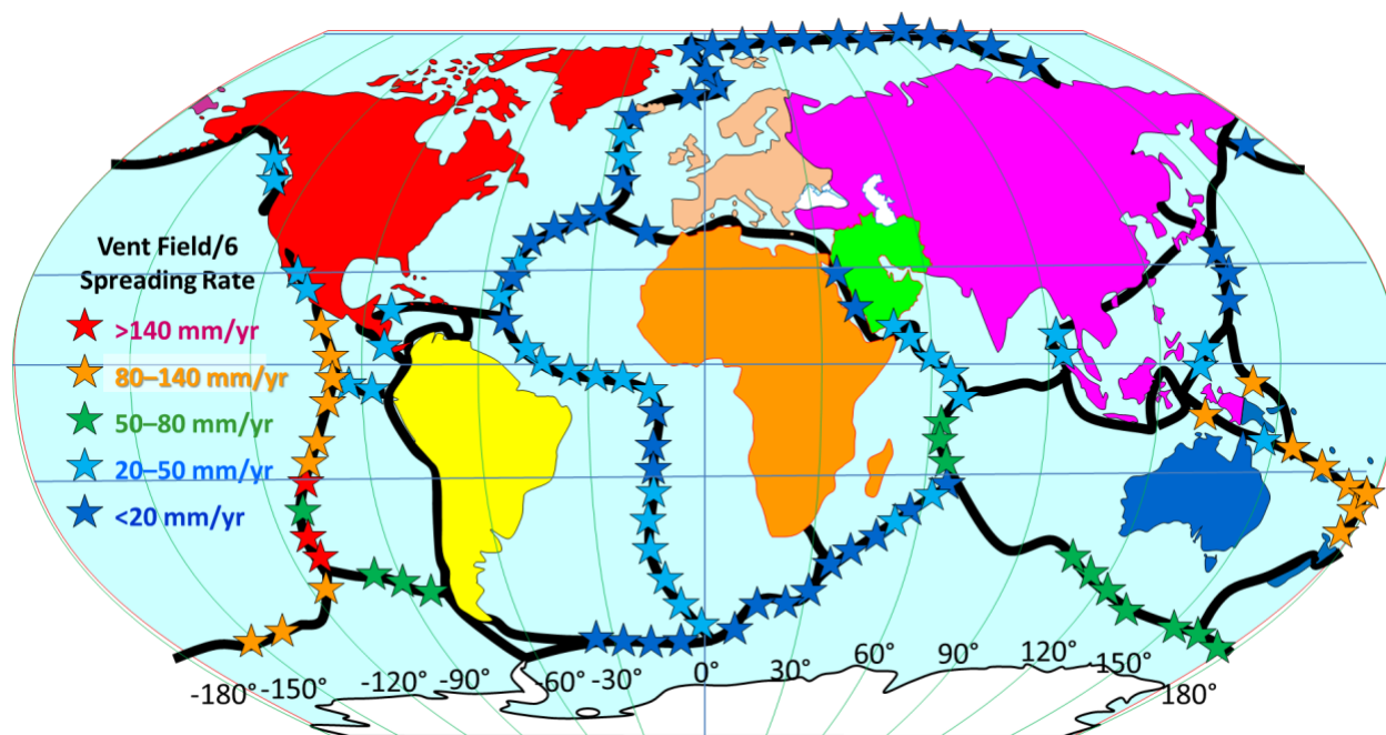
Figure 3 – Hydrothermal Vent Field Spreading Rates
