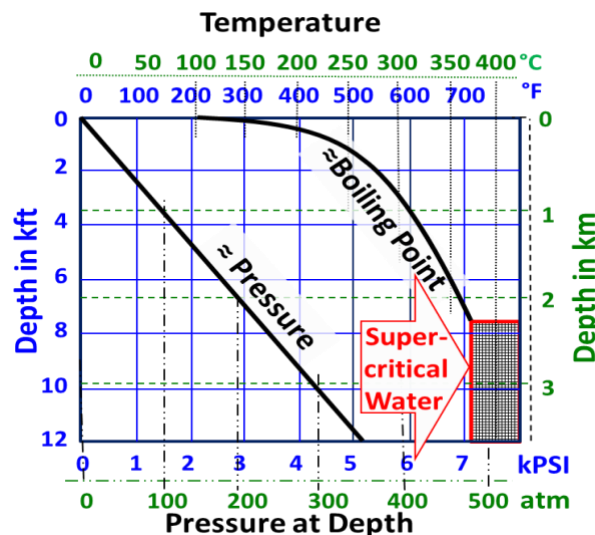
Figure 7 – Typical Pressure and Water State vs Ocean Depth
