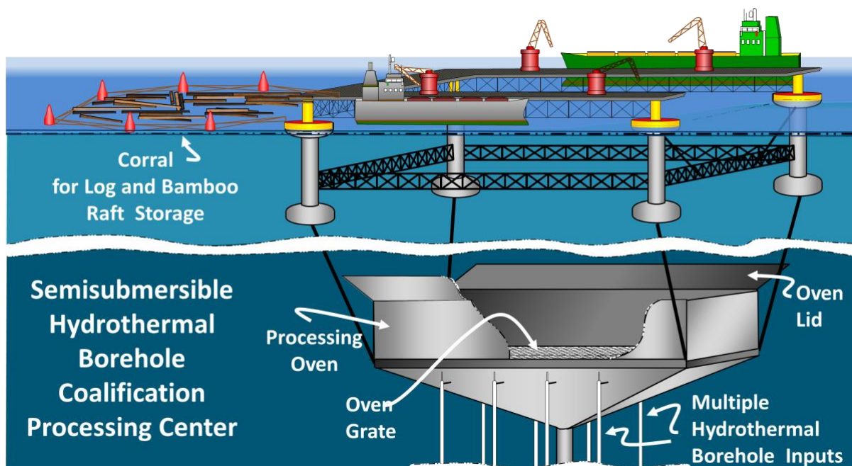
Figure 9 – Large Mid-Ocean Ridge DOCS Processing Center
